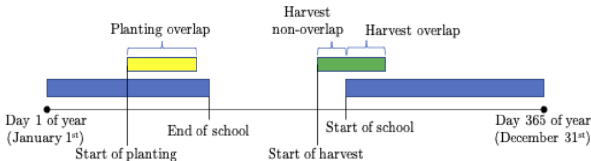
Figure A1: Defining overlap and non-overlap
